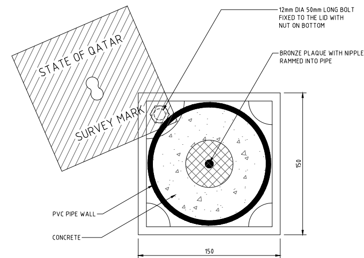
PLAN (LID OPEN)
