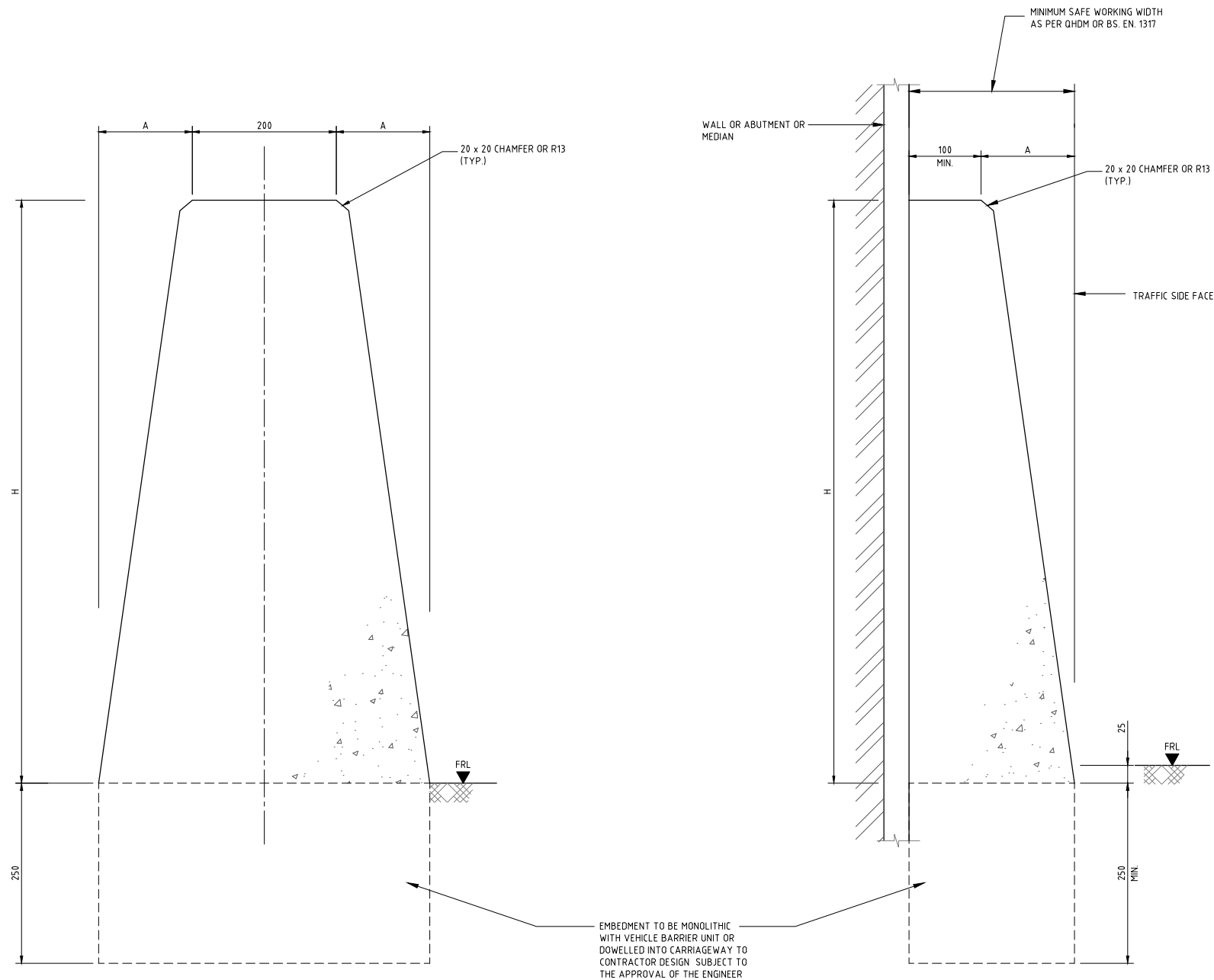
CONCRETE VBU (DOUBLE FACED)
