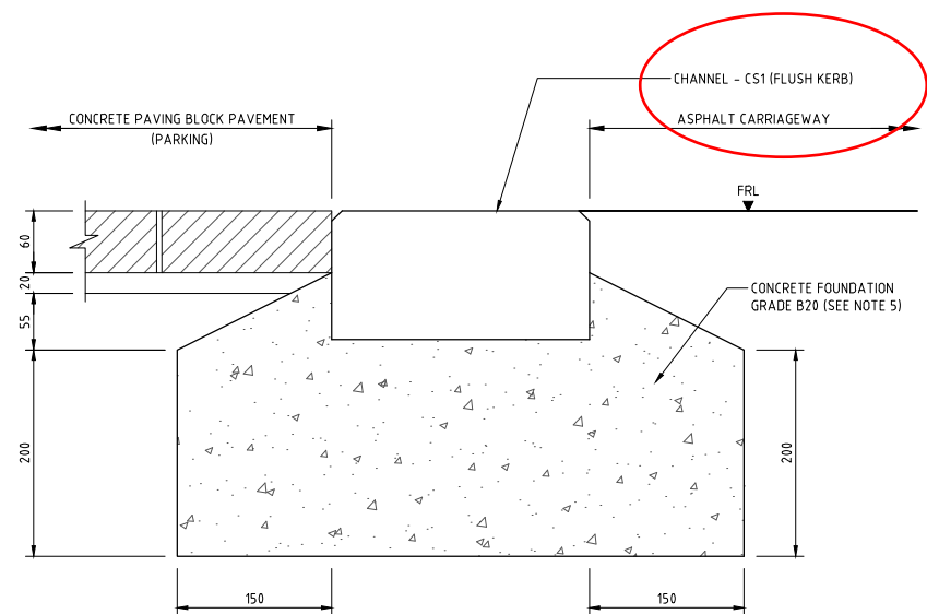
CHANNEL - CS1 (FLUSH KERB) IN CARRIAGEWAY MONOLITHIC FOUNDATION
