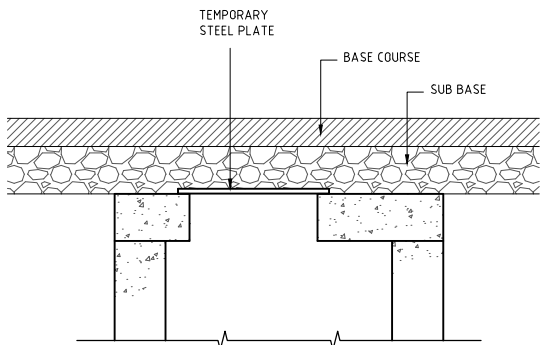
STEP 1 PLATING OVER MANHOLE OPENING
