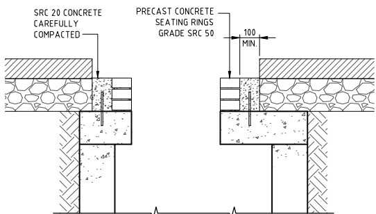
STEP 3 BUILD UP PRECAST SEATING RINGS AND CONCRETE IN PLACE REMOVE DEBRIS FROM MANHOLE
