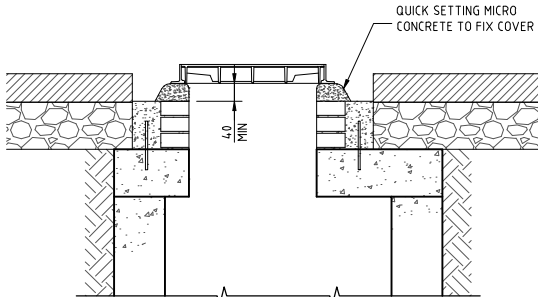
STEP 4 LAYING OF CONCRETE SEALING
