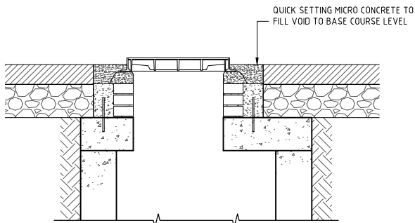
STEP 5 FIX MANHOLE COVER TO FINISHED WEARING COURSE LEVELS USING QUICK SETTING MICRO CONCRETE
