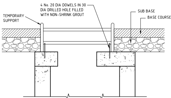
STEP 2 REMOVAL OF PLATE, TRIM EXCAVATION TEMPORARY SUPPORT, INSTALL DOWELS
