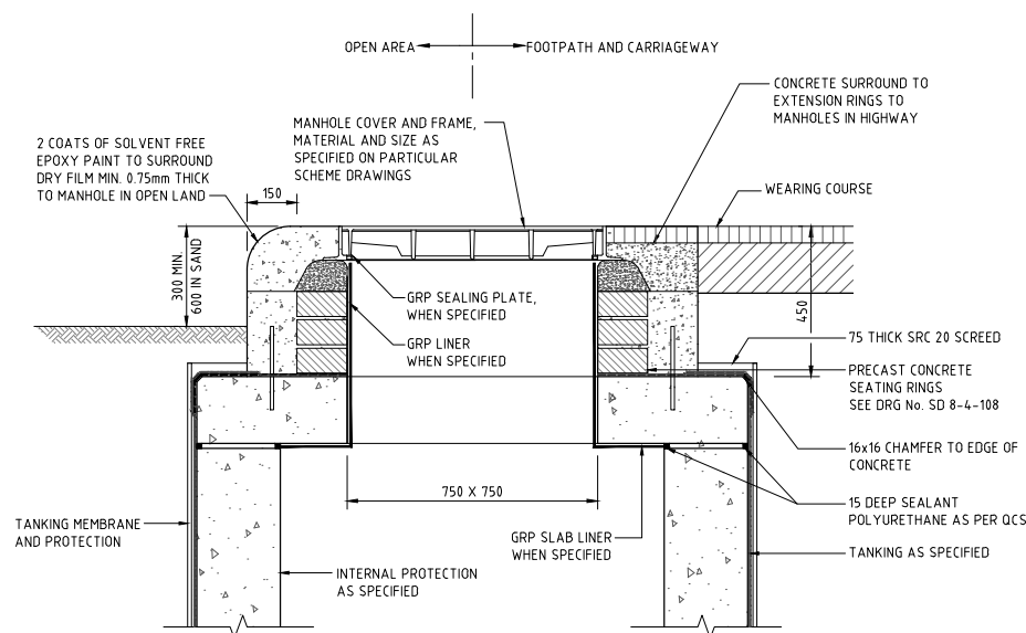
CONCRETE SURROUND TO MANHOLE CHAMBER ACCESS
