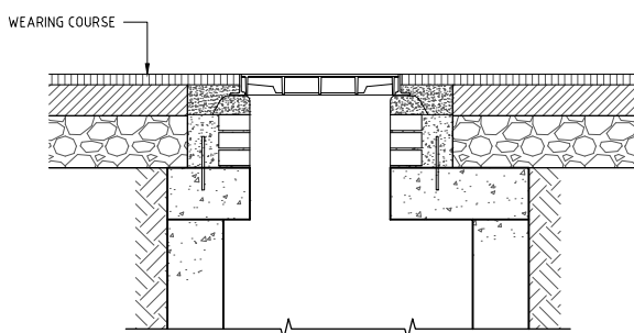
STEP 6 WEARING COURSE LAID
