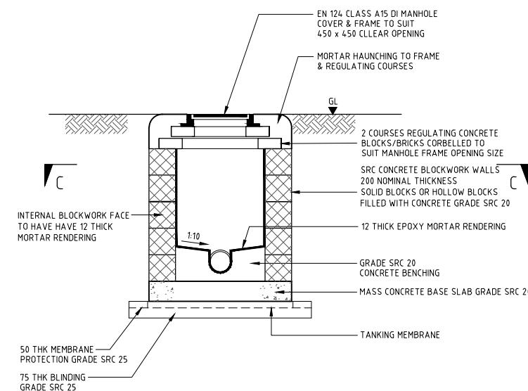
SECTION D-D CHAMBER TYPE 'C'
