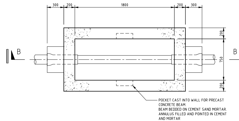
SECTION A-A CHAMBER TYPE 'B'
