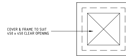
PLAN ON COVER
