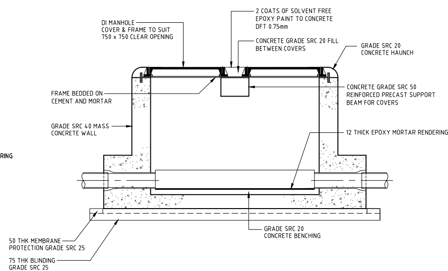
SECTION C-C CHAMBER TYPE 'B'
